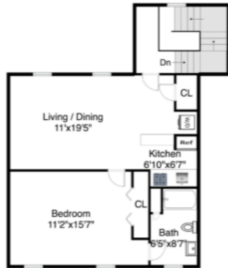
Garage - Second Floor Plan
